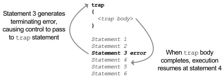
Figure 14.9 The flow of control when a trap statement is used. If there's a trap statement in scope, control transfers to the body of the trap statement where the error is processed.
