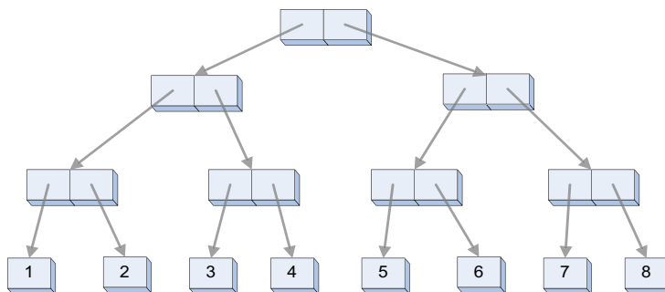
Figure 5.6 A binary tree (arrays of arrays of arrays)
