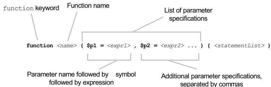
Figure 7.4 The more complex function definition syntax where initializer expressions are provided for each variable. Note that the initializers are constrained to be expressions, but, using the subexpression notation, you can put anything here.
