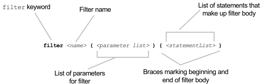
Figure 7.6 Defining a filter in PowerShell. The syntax is identical to the basic function definition except that it uses the filter keyword instead of the function keyword.
