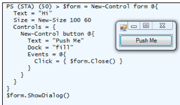
Figure 17.9 An example using the WPISForms module. Both the code and the resulting window are shown here.
