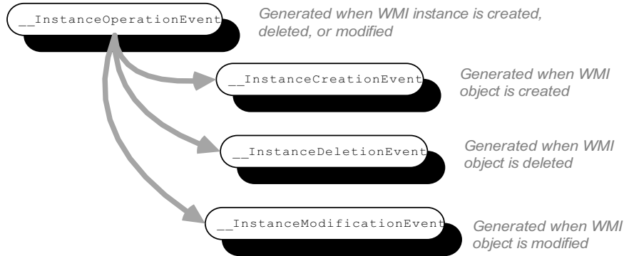
Figure 20.5 The class hierarchy for the WMI instance operation event class. These events are generated when a WMI object is created, deleted, or modified. The base event class is triggered for all three.
