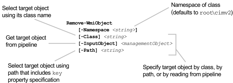
Figure 19.7 The Remove-WmiObject cmdlet allows you to remove objects from the system using WMI.
