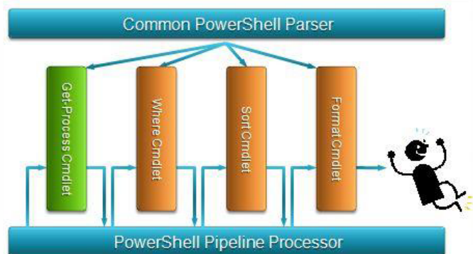
Figure 11.3 Objects flow through a pipeline one at a time. A common parser constructs each of the command objects and then starts the pipeline processor, stepping each object through all stages of the pipeline.
