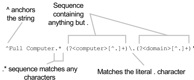
Figure 4.8 This is an example of a regular expression pattern that uses the named submatch capability. When this expression is used with the -match operator, instead of using simple numeric indexes in the $matches variable for the substrings, the names will be used.
