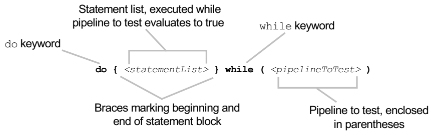
Figure 6.6 The PowerShell do-while loop statement syntax
