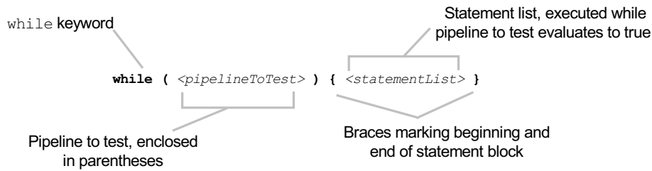
Figure 6.5 The PowerShell while loop statement syntax
